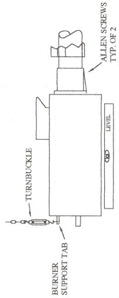
BURNER INSTALLATION DETAIL
